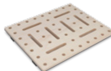
REAR WALL WORKTOP WO RW 750 Ref. No. 1000004365 Dimensions (WxHxD): 572 x 685 x 78 mm
