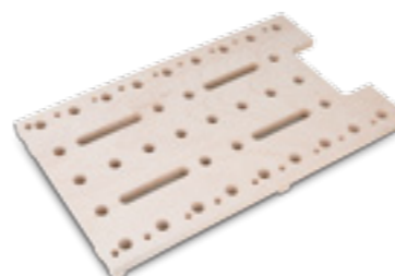
SIDE WALL WORKTOP WO AP SW 750 Ref. No. 1000004366 Dimensions (WxHxD): 346 x 552 x 27 mm
